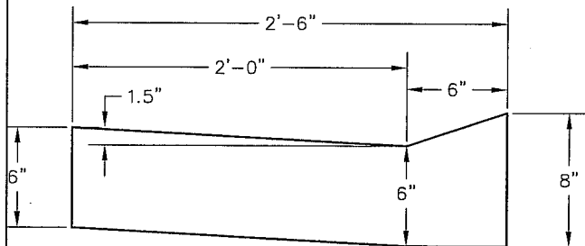
DRIVEWAY ENTRANCE CURB SECTION
