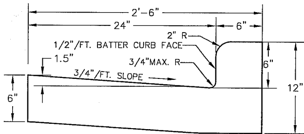
6" CURB TYPE D SECTION
