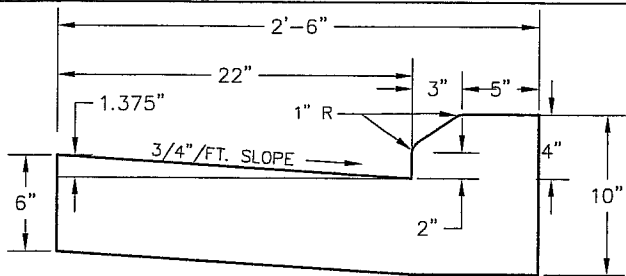
4" SLOPED CURB TYPE J SECTION
