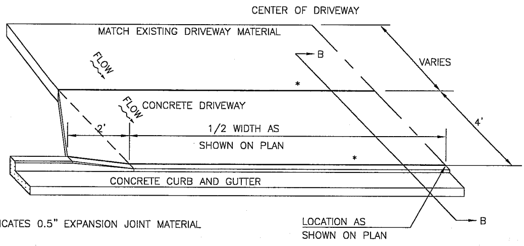
FRONT PITCH DRIVEWAY RECONSTRUCTION TYPE 1 DRIVEWAY
