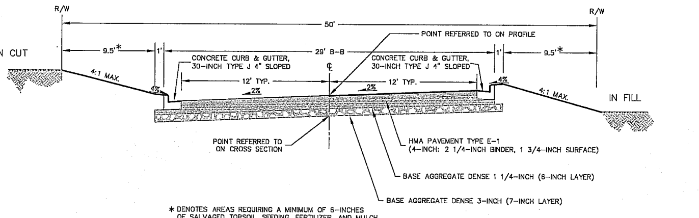
TYPICAL CROSS SECTION POCAHONTAS DRIVE STATION 64+50 TO STATION 66+00
