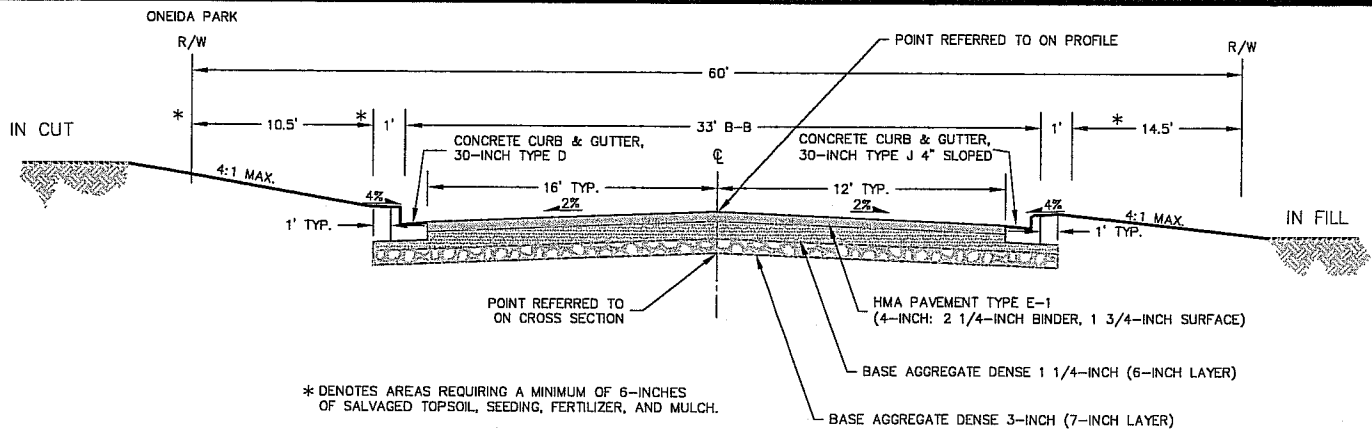
TYPICAL CROSS SECTION TECUMSEH AVENUE STATION 10+25 TO STATION 19+38
