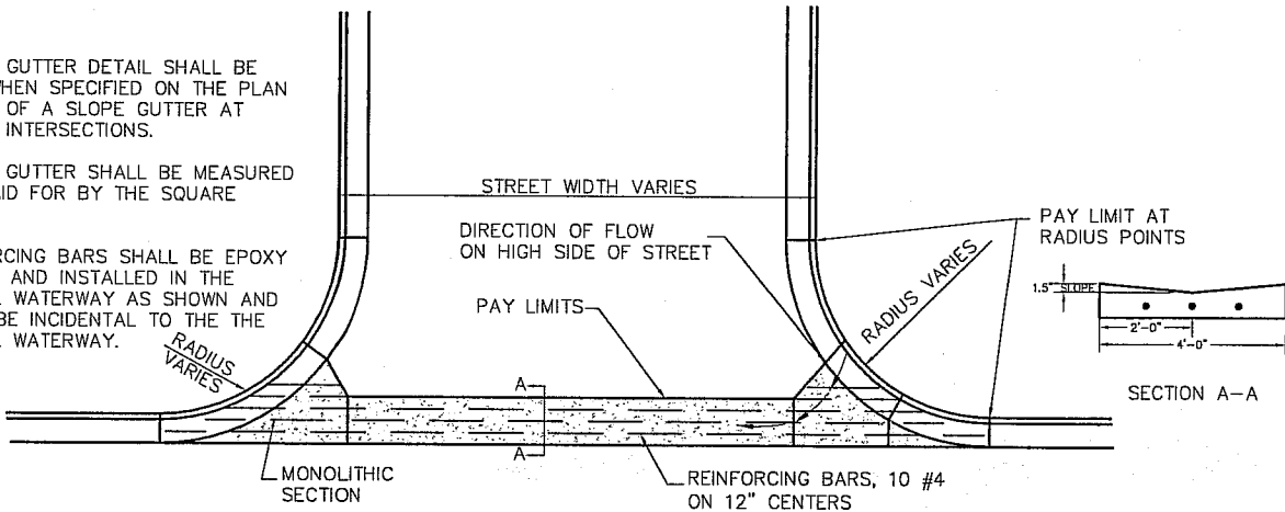
VALLEY GUTTER DETAIL NISHISHIN TRAIL & NISHISHIN TRAIL NE INTERSECTION
