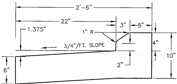
REJECT CURB SECTION
