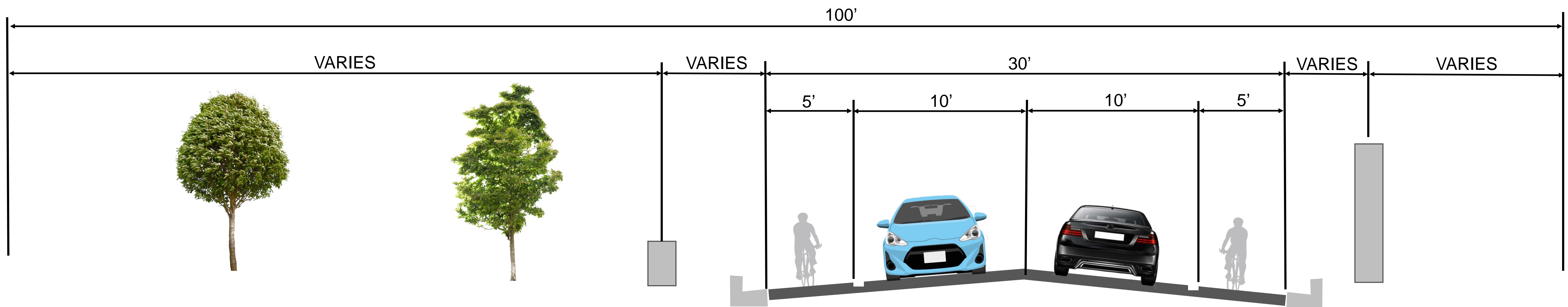
Option 1 - Proposed South Winnequah Road Northern Typical Section
