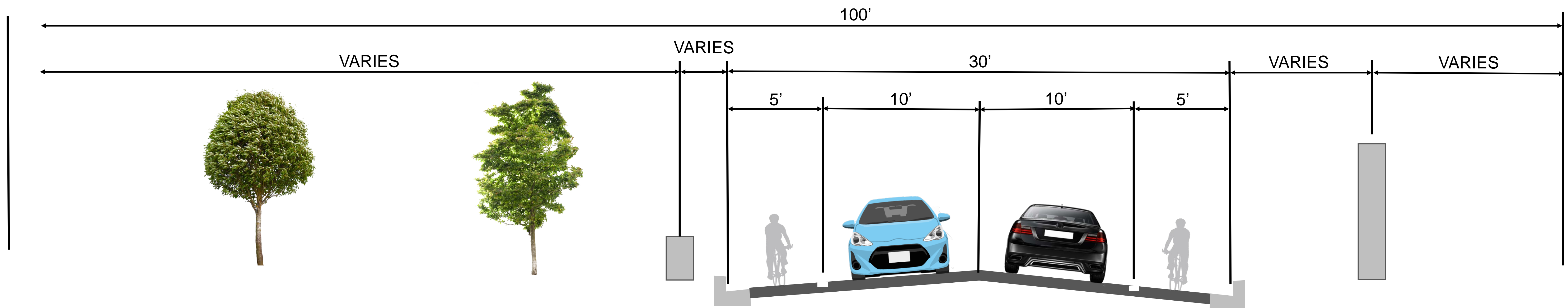
Option 2 - Proposed South Winnequah Road Northern Typical Section
