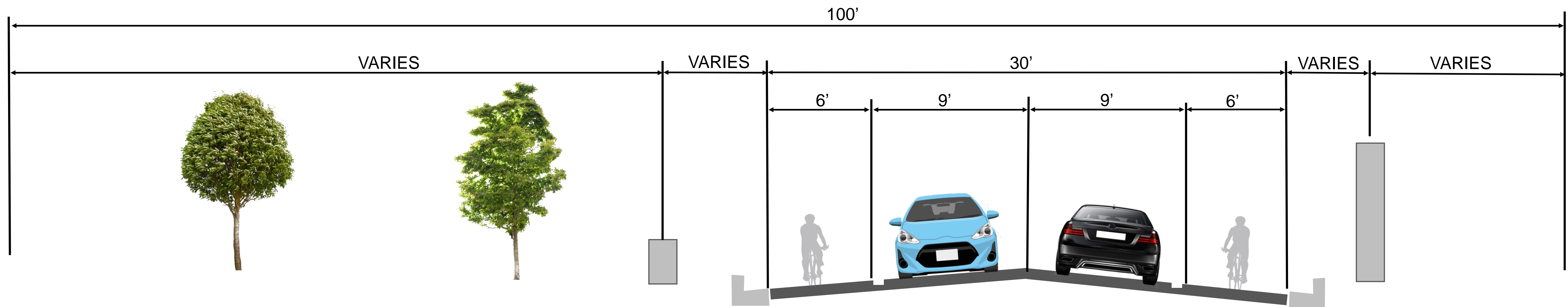
Existing South Winnequah Road Northern Typical Section
