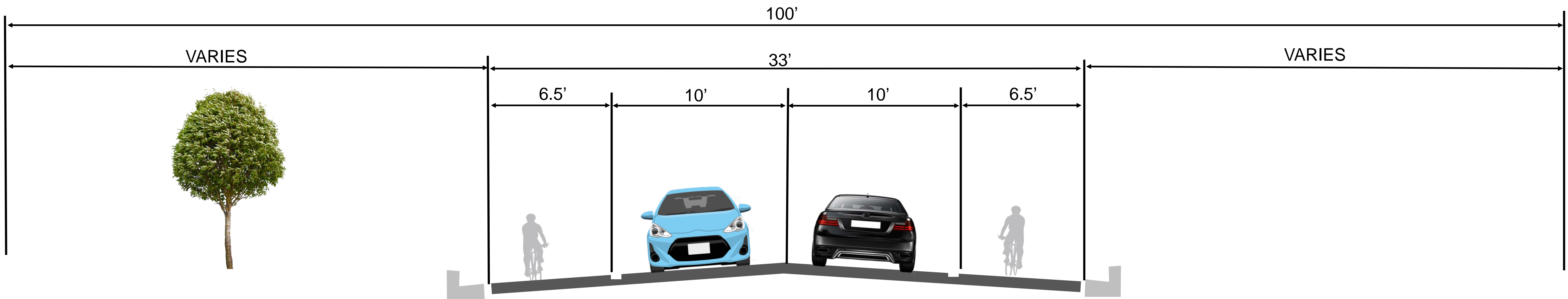
Options 1 & 2 - Proposed South Winnequah Road Southern Typical Section
