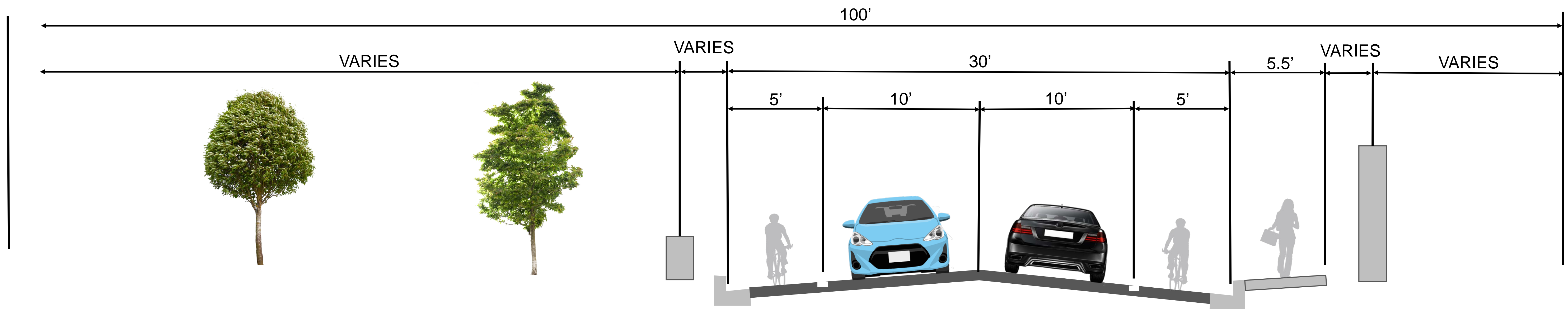
Option 3 - Proposed South Winnequah Road Northern Typical Section
