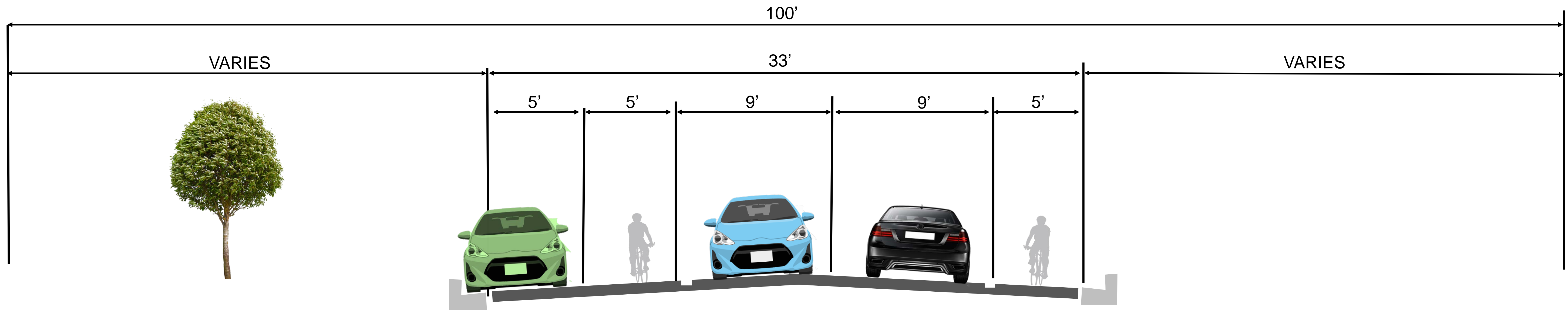
Existing South Winnequah Road Southern Typical Section
