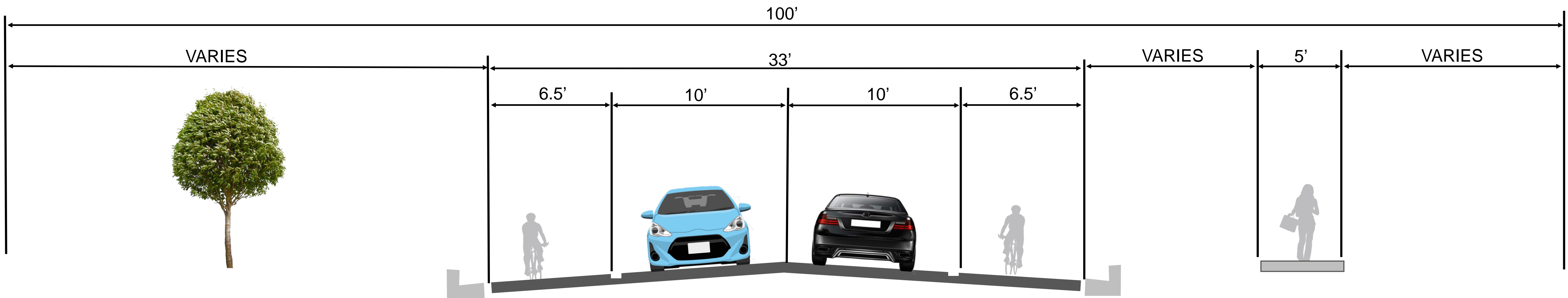
Option 3 - Proposed South Winnequah Road Southern Typical Section
