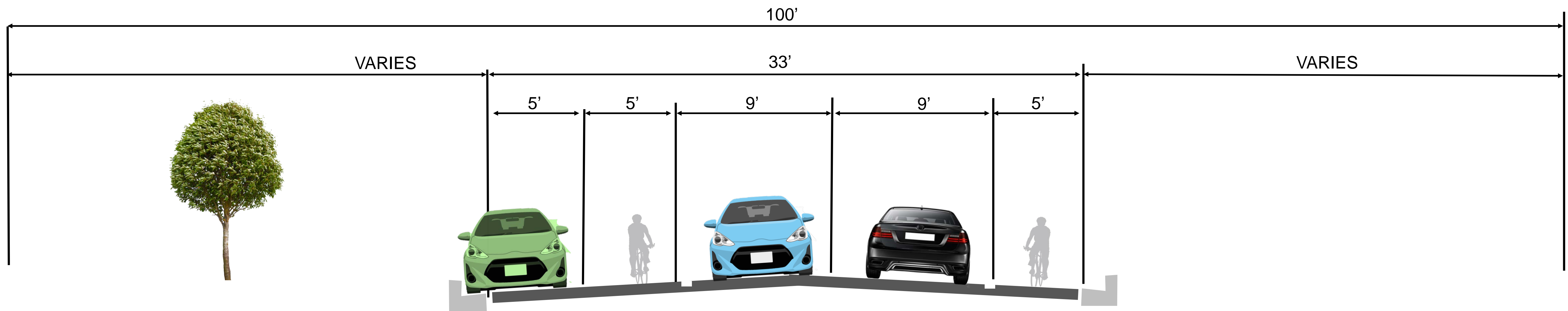
Existing South Winnequah Road Southern Typical Section
